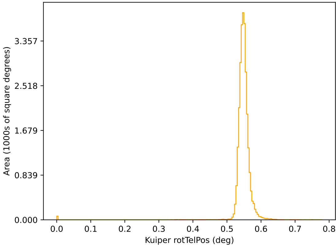
too_elab_r64_d2_giz_v3.4_10yrs r: Kuiper rotTelPos
