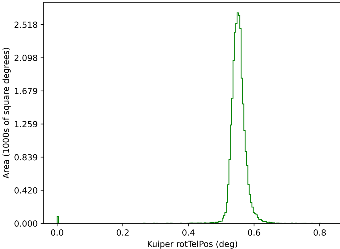
too_elab_r64_d2_giz_v3.4_10yrs g: Kuiper rotTelPos
