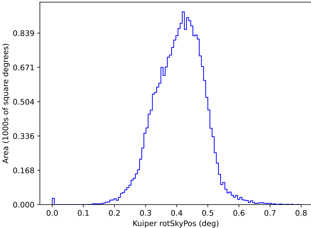
too_elab_r64_d2_giz_v3.4_10yrs y: Kuiper rotSkyPos
