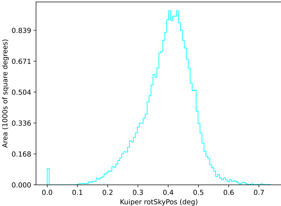
too_elab_r64_d2_giz_v3.4_10yrs u: Kuiper rotSkyPos
