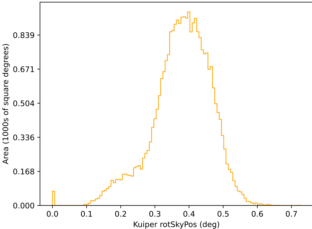
too_elab_r64_d2_giz_v3.4_10yrs r: Kuiper rotSkyPos
