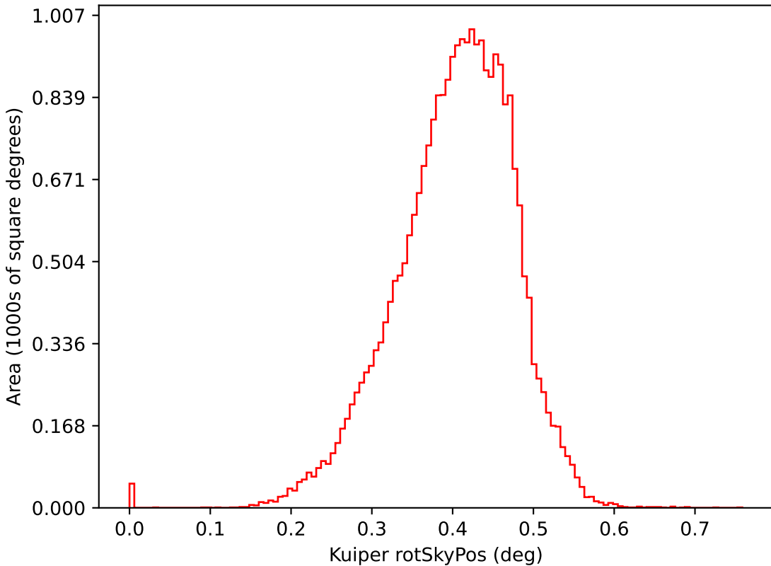
too_elab_r64_d2_giz_v3.4_10yrs i: Kuiper rotSkyPos
