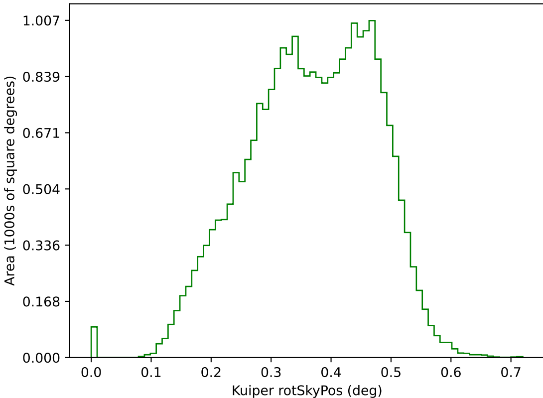
too_elab_r64_d2_giz_v3.4_10yrs g: Kuiper rotSkyPos
