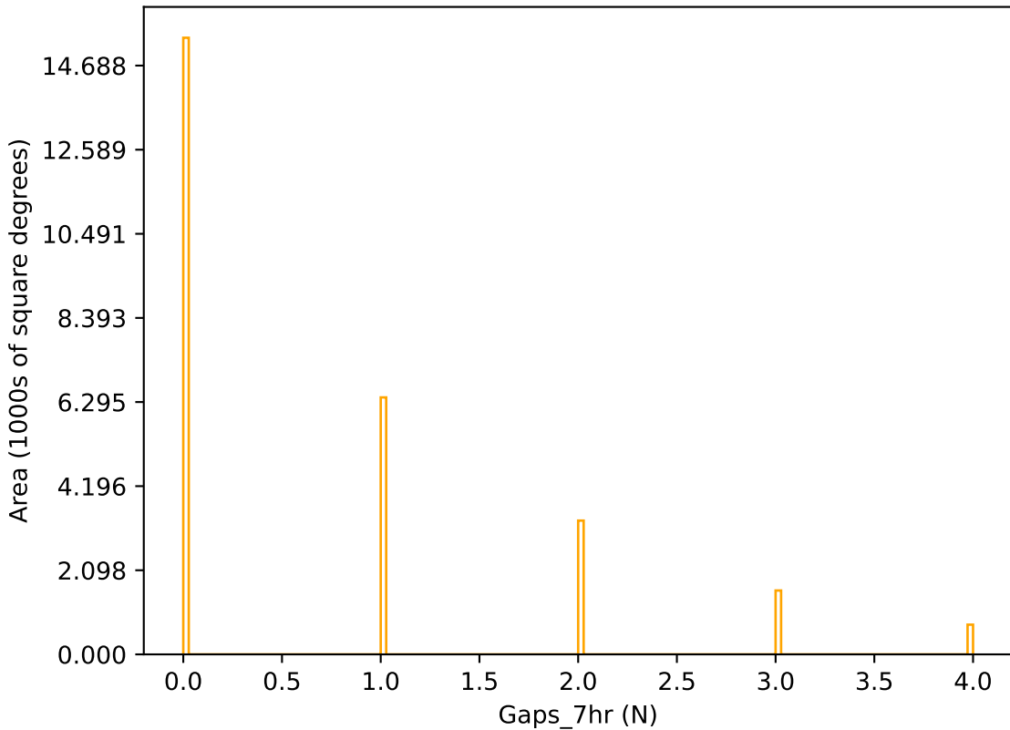
too_elab_r64_d2_giz_v3.4_10yrs r band: Gaps_7hr
