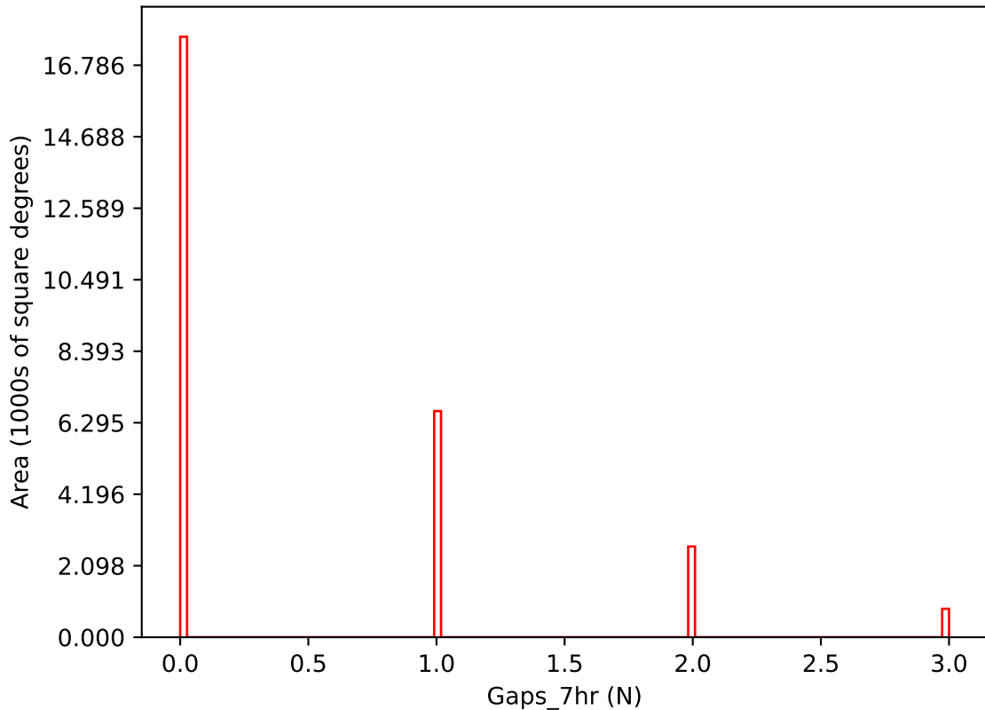
too_elab_r64_d2_giz_v3.4_10yrs i band: Gaps_7hr
