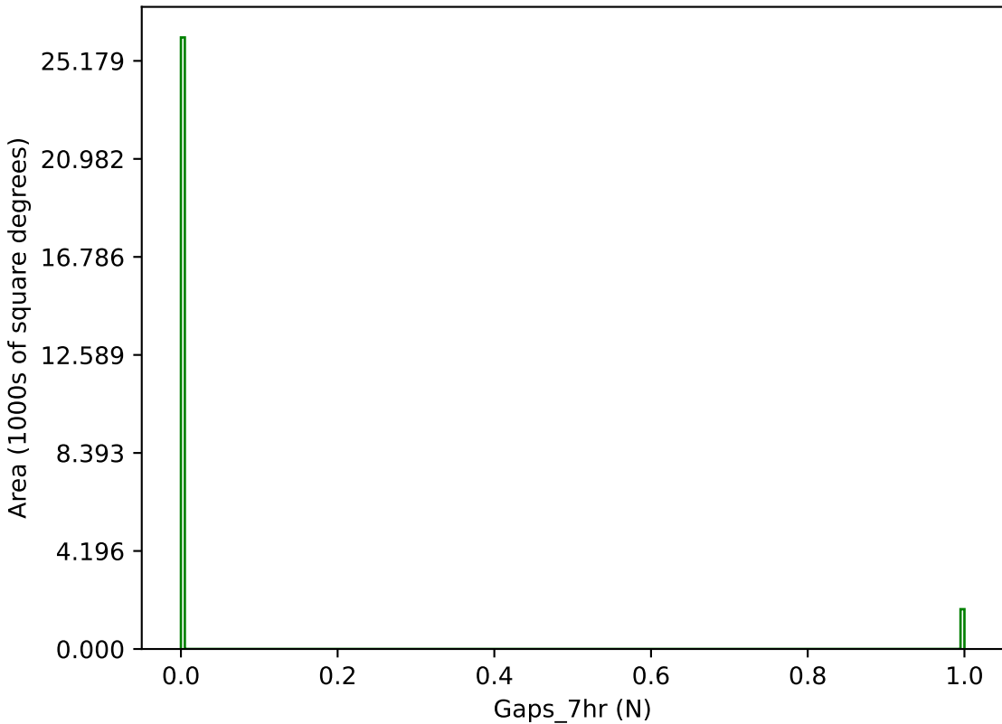
too_elab_r64_d2_giz_v3.4_10yrs g band: Gaps_7hr
