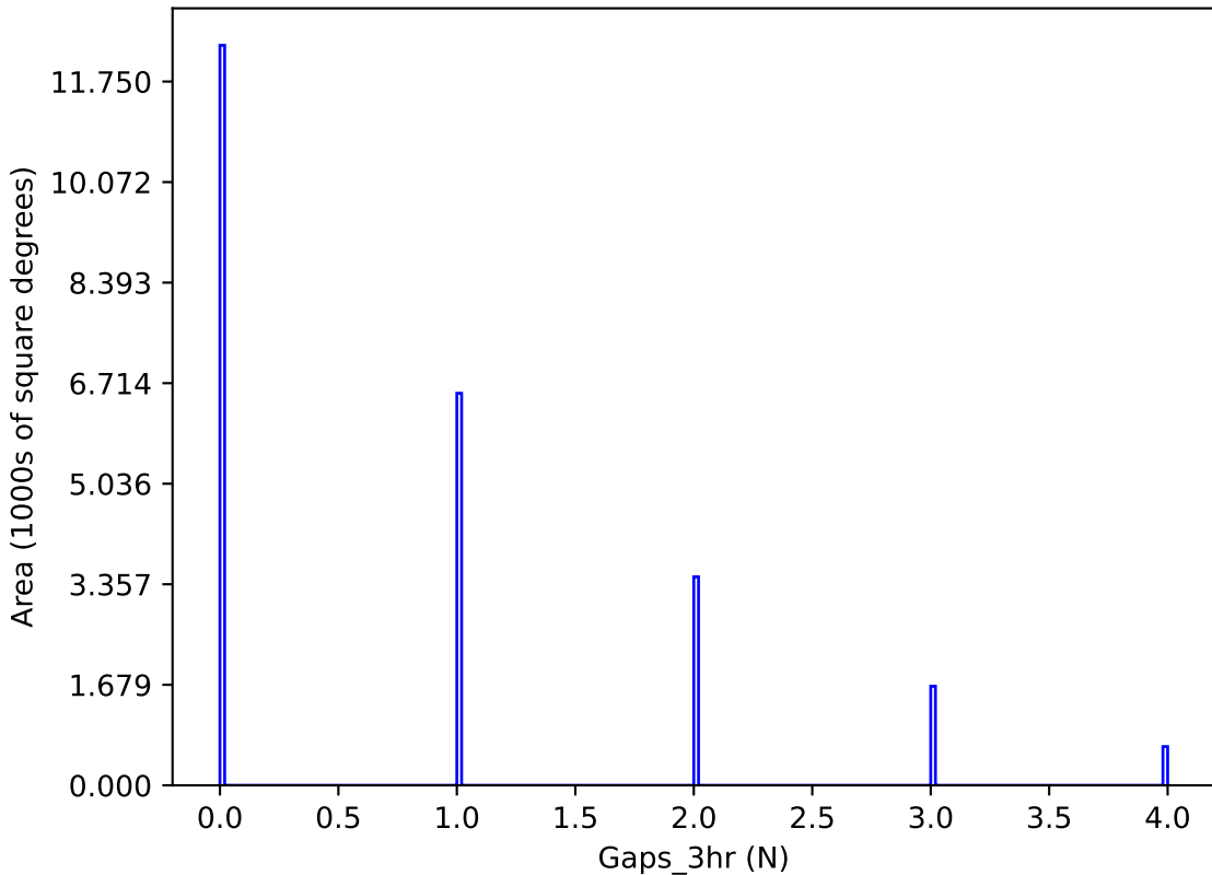
too_elab_r64_d2_giz_v3.4_10yrs y band: Gaps_3hr
