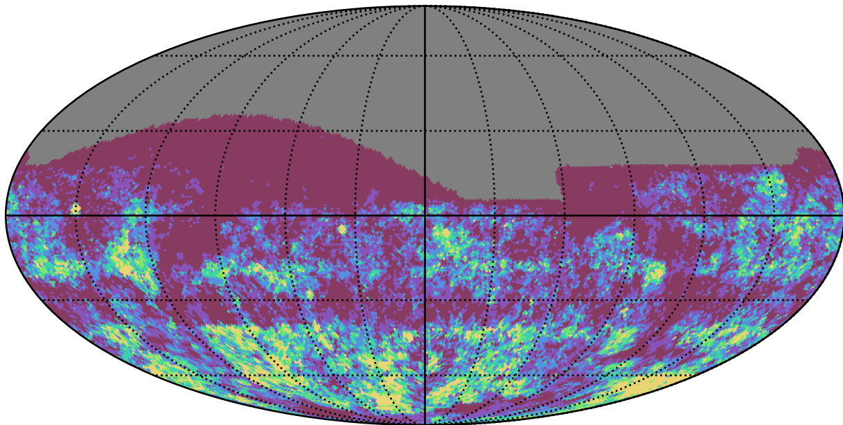
too_elab_r64_d2_giz_v3.4_10yrs r band: Gaps_3hr
