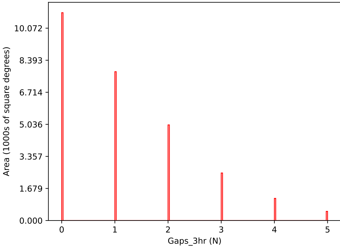
too_elab_r64_d2_giz_v3.4_10yrs i band: Gaps_3hr
