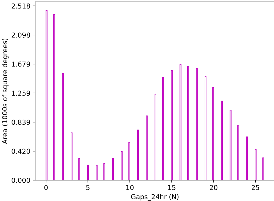
too_elab_r64_d2_giz_v3.4_10yrs z band: Gaps_24hr
