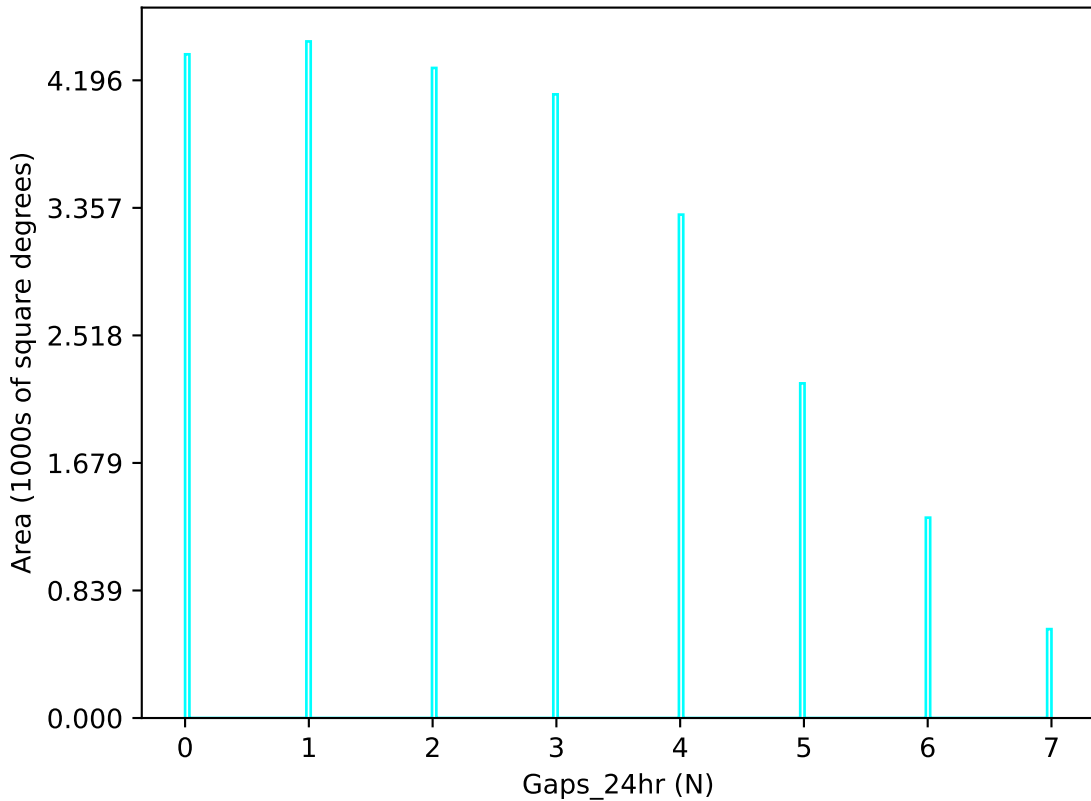
too_elab_r64_d2_giz_v3.4_10yrs u band: Gaps_24hr
