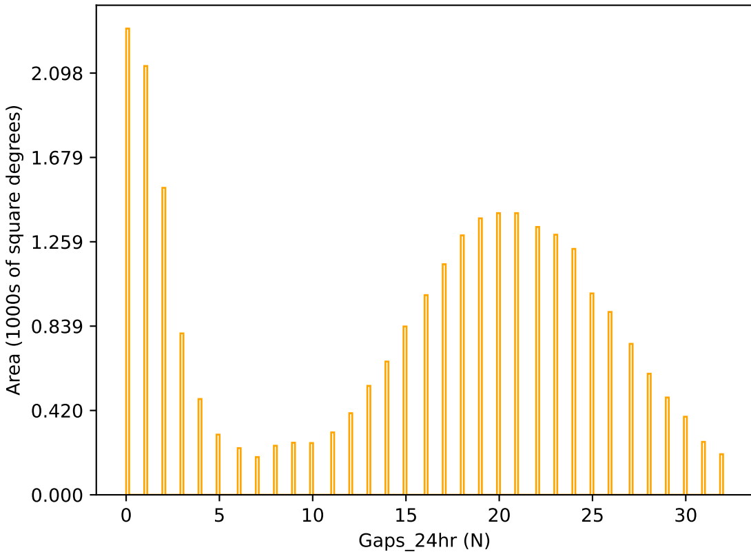
too_elab_r64_d2_giz_v3.4_10yrs r band: Gaps_24hr
