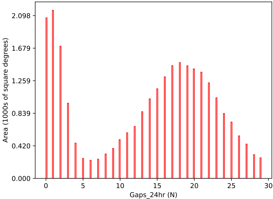
too_elab_r64_d2_giz_v3.4_10yrs i band: Gaps_24hr
