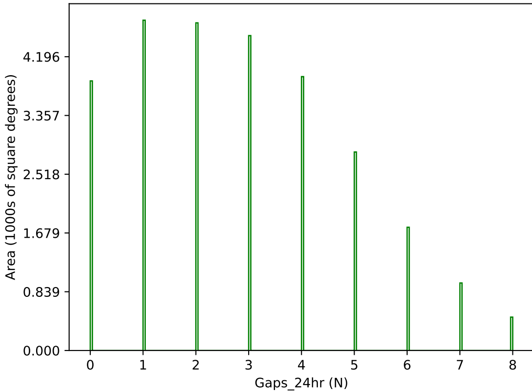
too_elab_r64_d2_giz_v3.4_10yrs g band: Gaps_24hr
