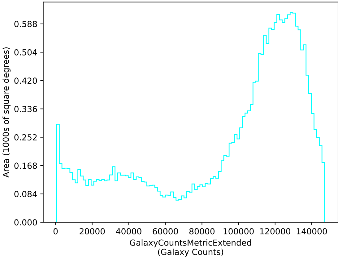
too_elab_r64_d2_giz_v3.4_10yrs u: GalaxyCountsMetricExtended
