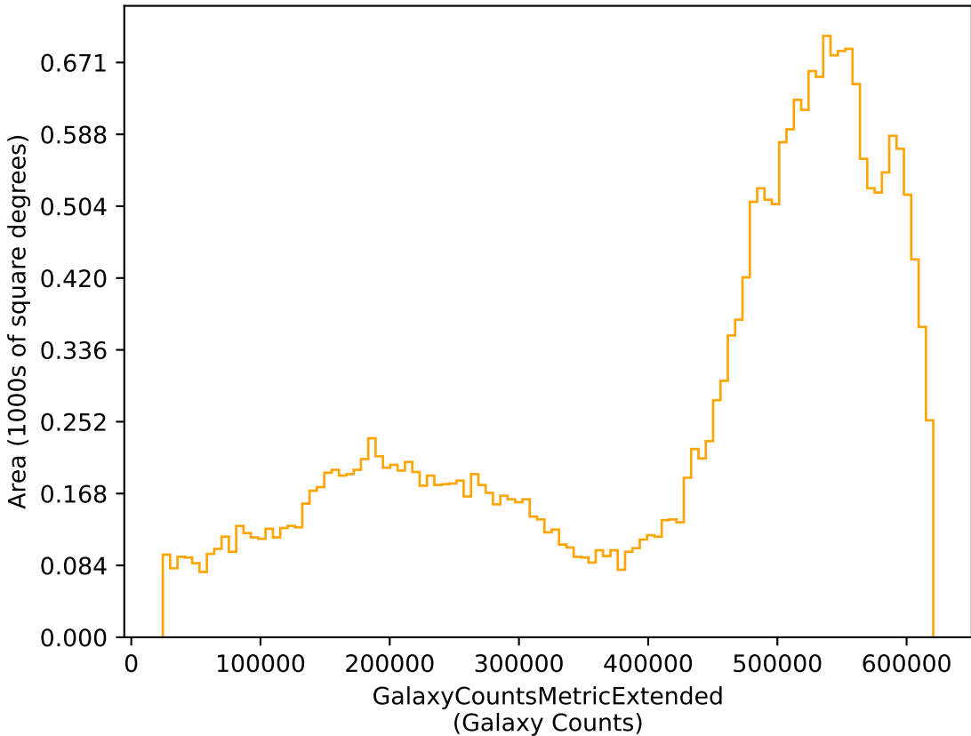
too_elab_r64_d2_giz_v3.4_10yrs r: GalaxyCountsMetricExtended
