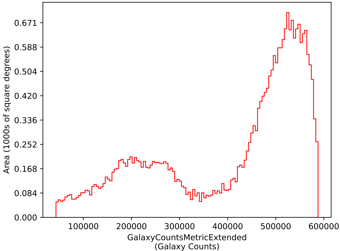
too_elab_r64_d2_giz_v3.4_10yrs i: GalaxyCountsMetricExtended
