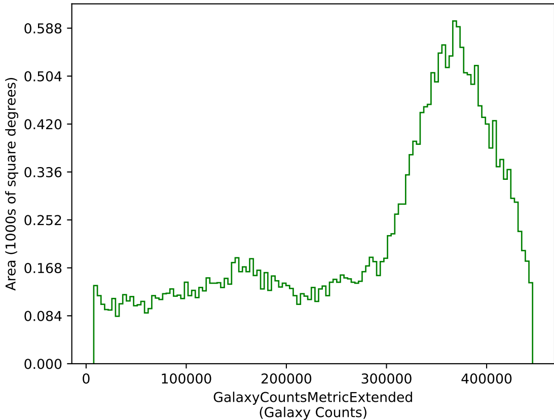
too_elab_r64_d2_giz_v3.4_10yrs g: GalaxyCountsMetricExtended
