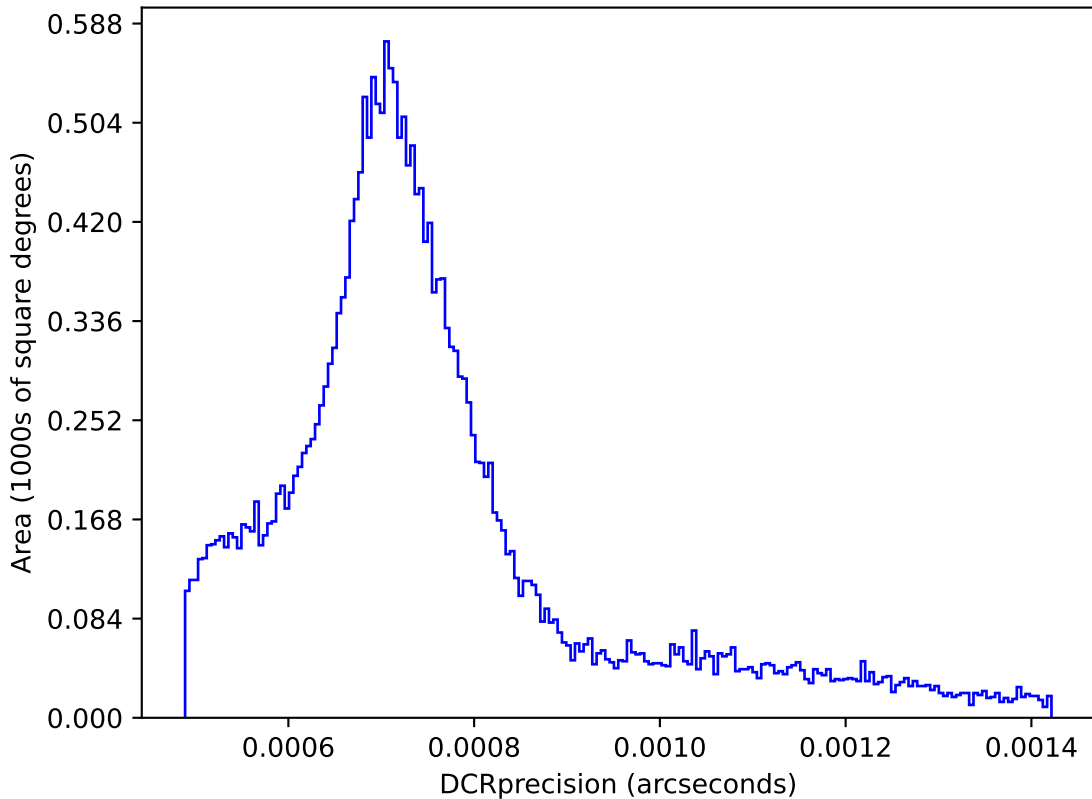
too_elab_r64_d2_giz_v3.4_10yrs : DCRprecision
