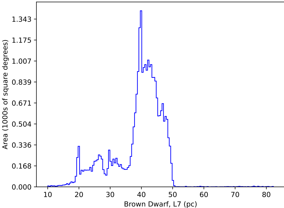
too_elab_r64_d2_giz_v3.4_10yrs : Brown Dwarf, L7
