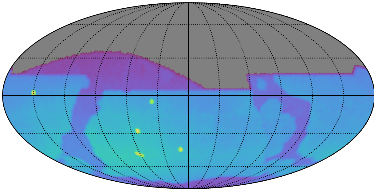
too_elab_r64_d2_giz_v3.4_10yrs : Brown Dwarf, L4
