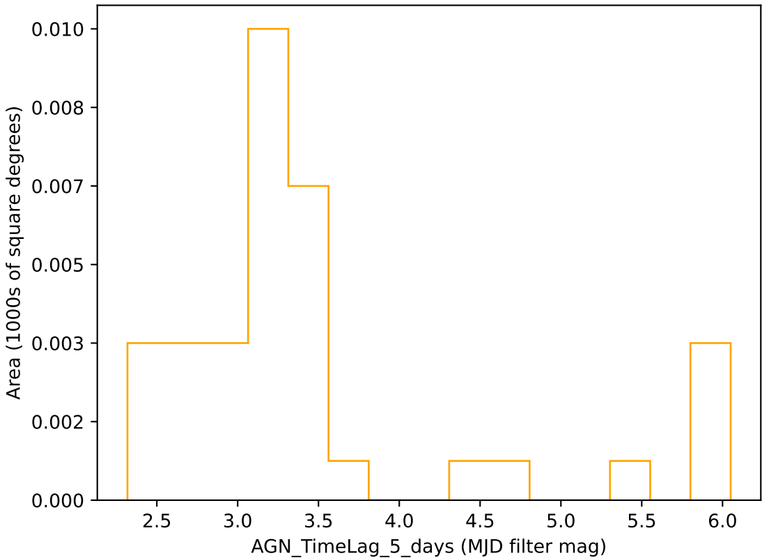
too_elab_r64_d2_giz_v3.4_10yrs r band: AGN_TimeLag_5_days
