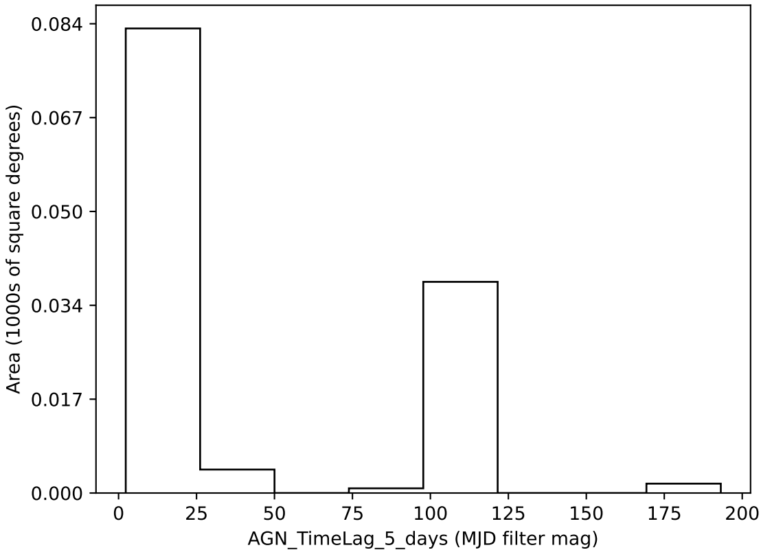
too_elab_r64_d2_giz_v3.4_10yrs all bands: AGN_TimeLag_5_days
