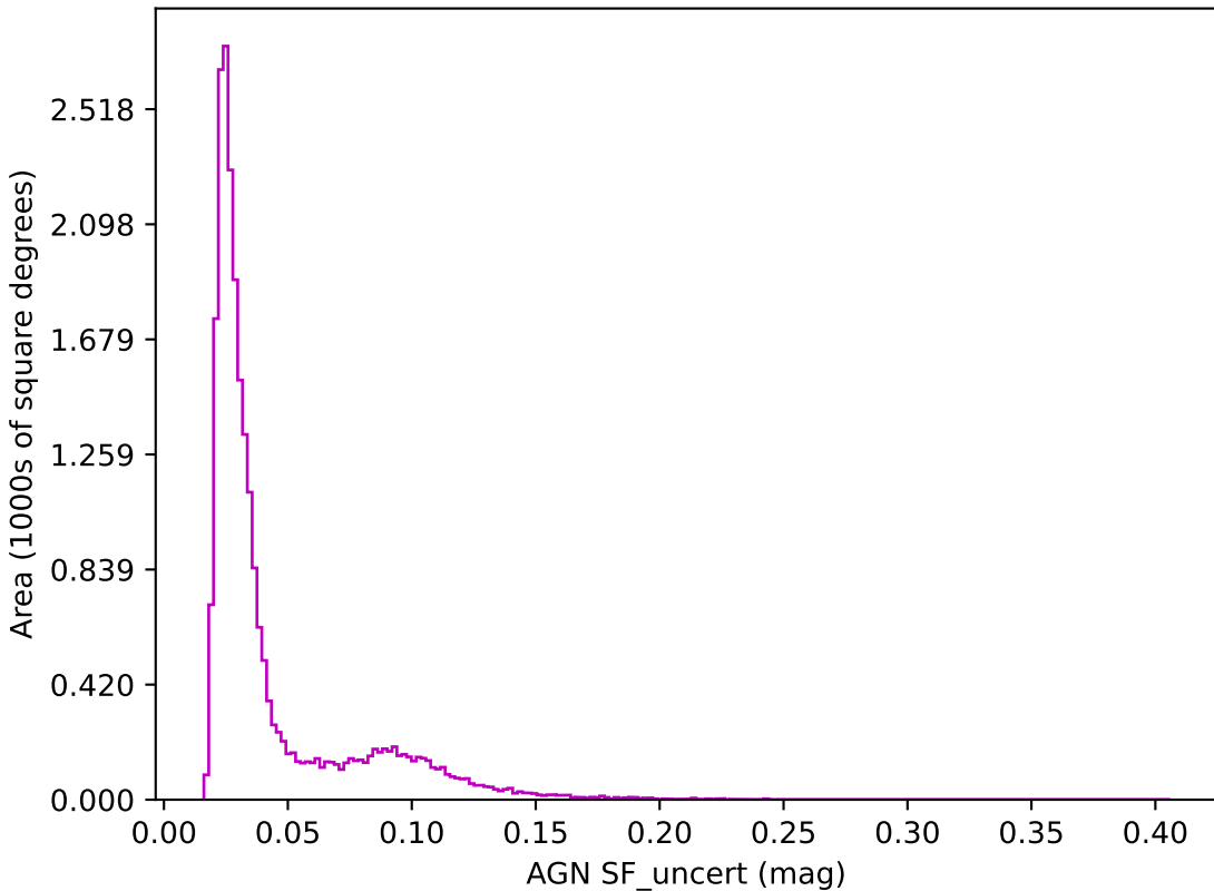
too_elab_r64_d2_giz_v3.4_10yrs z band: AGN SF_uncert
