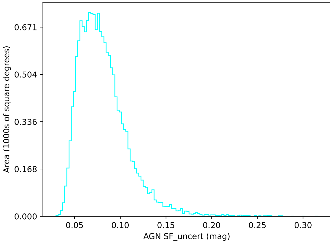
too_elab_r64_d2_giz_v3.4_10yrs u band: AGN SF_uncert
