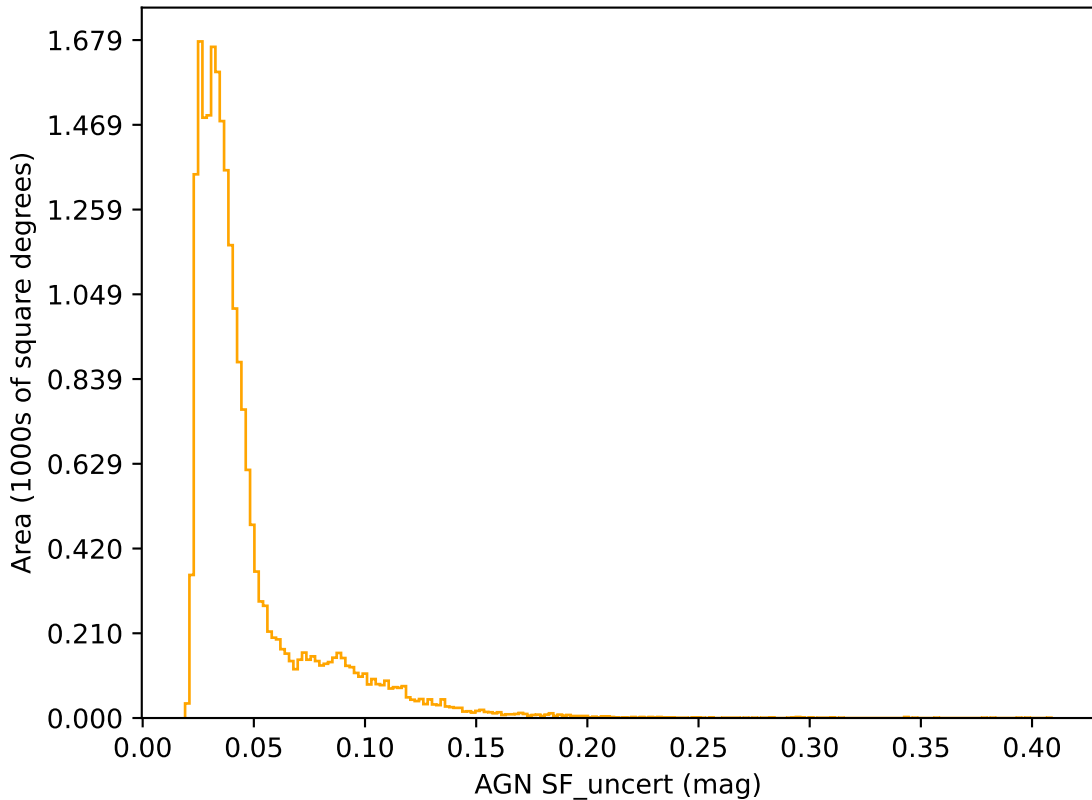
too_elab_r64_d2_giz_v3.4_10yrs r band: AGN SF_uncert
