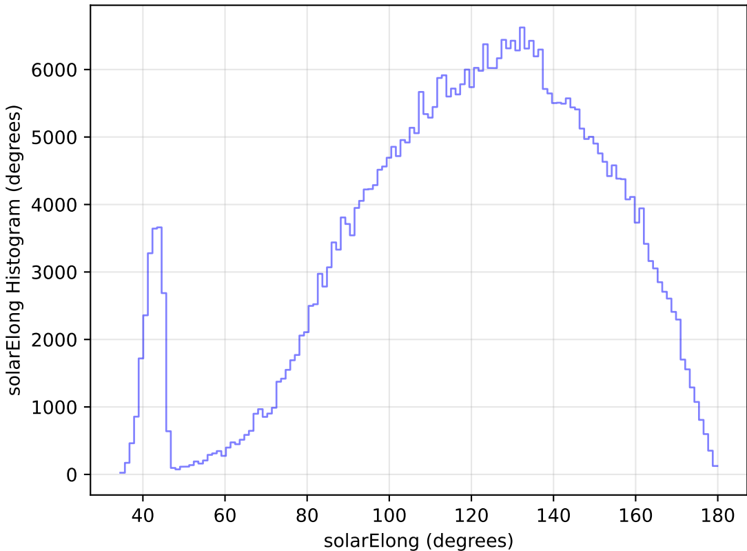
too_elab_r64_d2_giz_v3.4_10yrs WFD z band: solarElong Histogram
