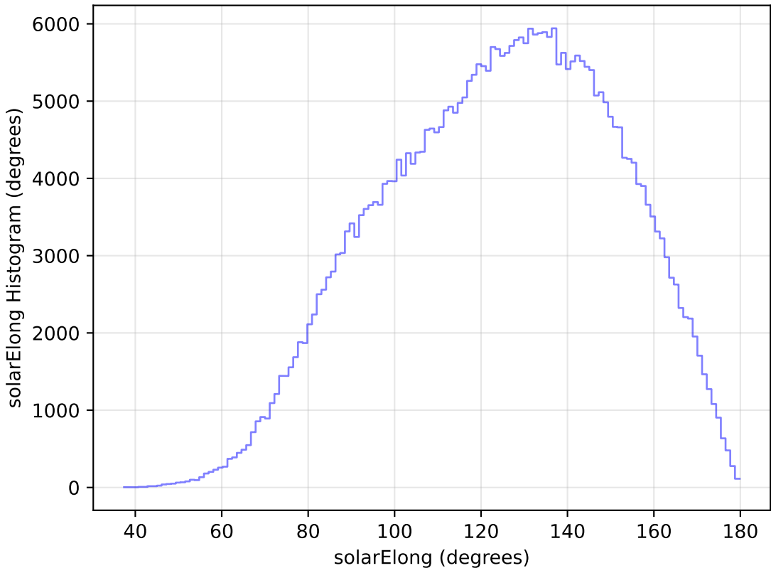
too_elab_r64_d2_giz_v3.4_10yrs WFD y band: solarElong Histogram
