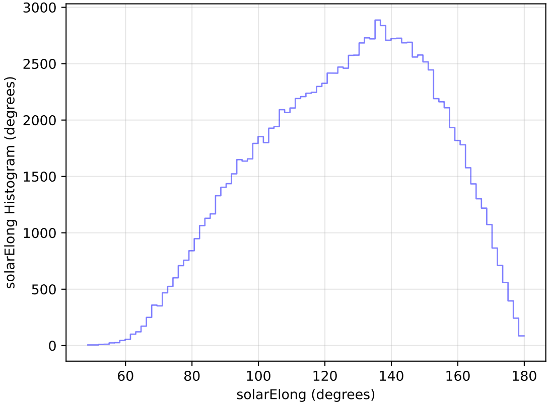
too_elab_r64_d2_giz_v3.4_10yrs WFD u band: solarElong Histogram
