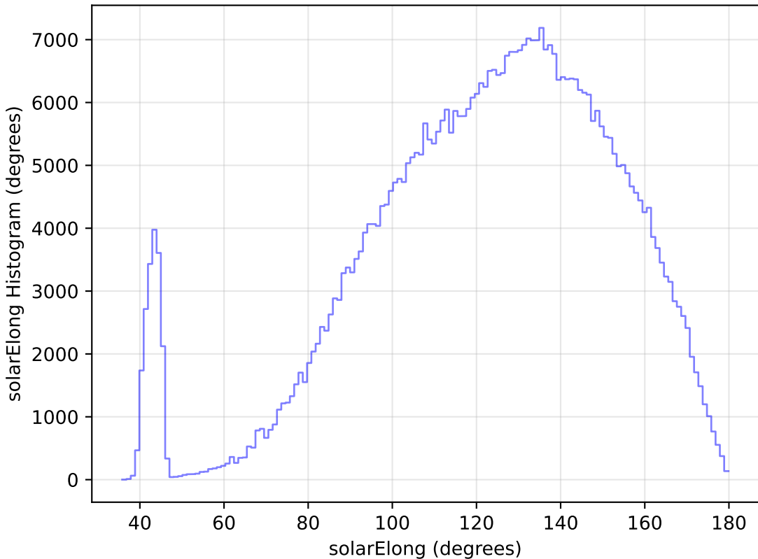
too_elab_r64_d2_giz_v3.4_10yrs WFD r band: solarElong Histogram
