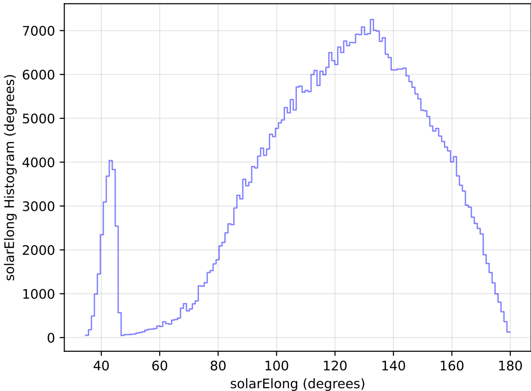
too_elab_r64_d2_giz_v3.4_10yrs WFD i band: solarElong Histogram
