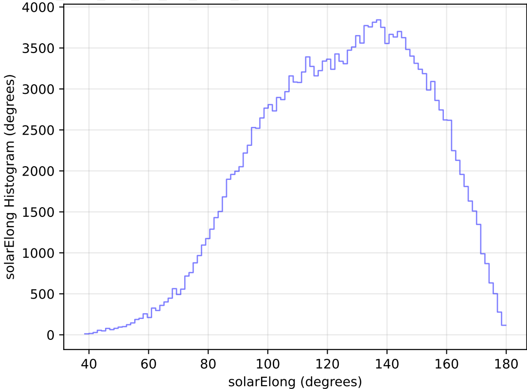
too_elab_r64_d2_giz_v3.4_10yrs WFD g band: solarElong Histogram
