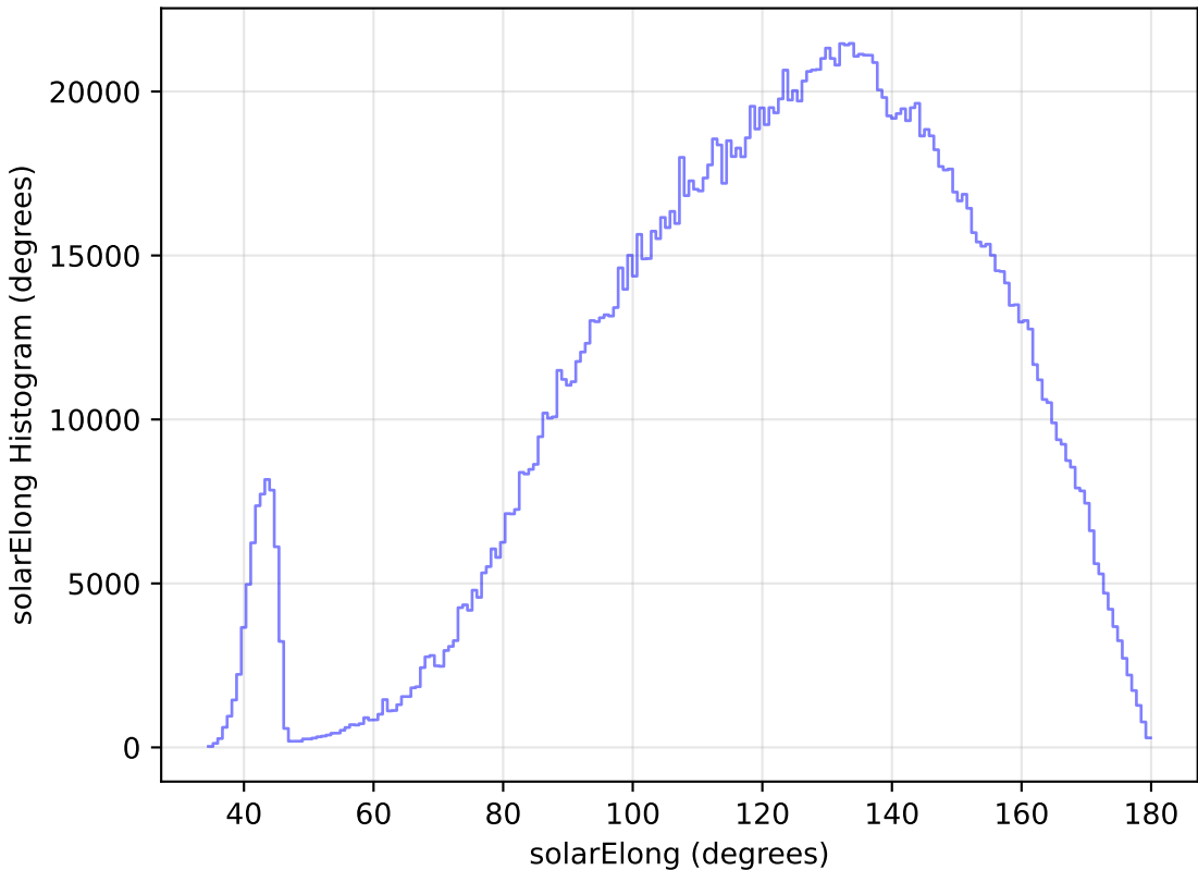
too_elab_r64_d2_giz_v3.4_10yrs WFD all bands: solarElong Histogram
