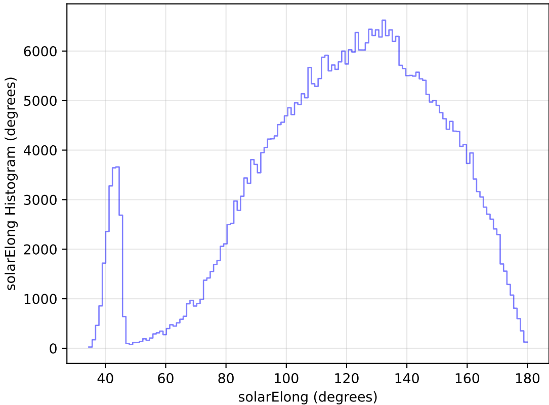
too_elab_r64_d2_giz_v3.4_10yrs All sky z band: solarElong Histogram
