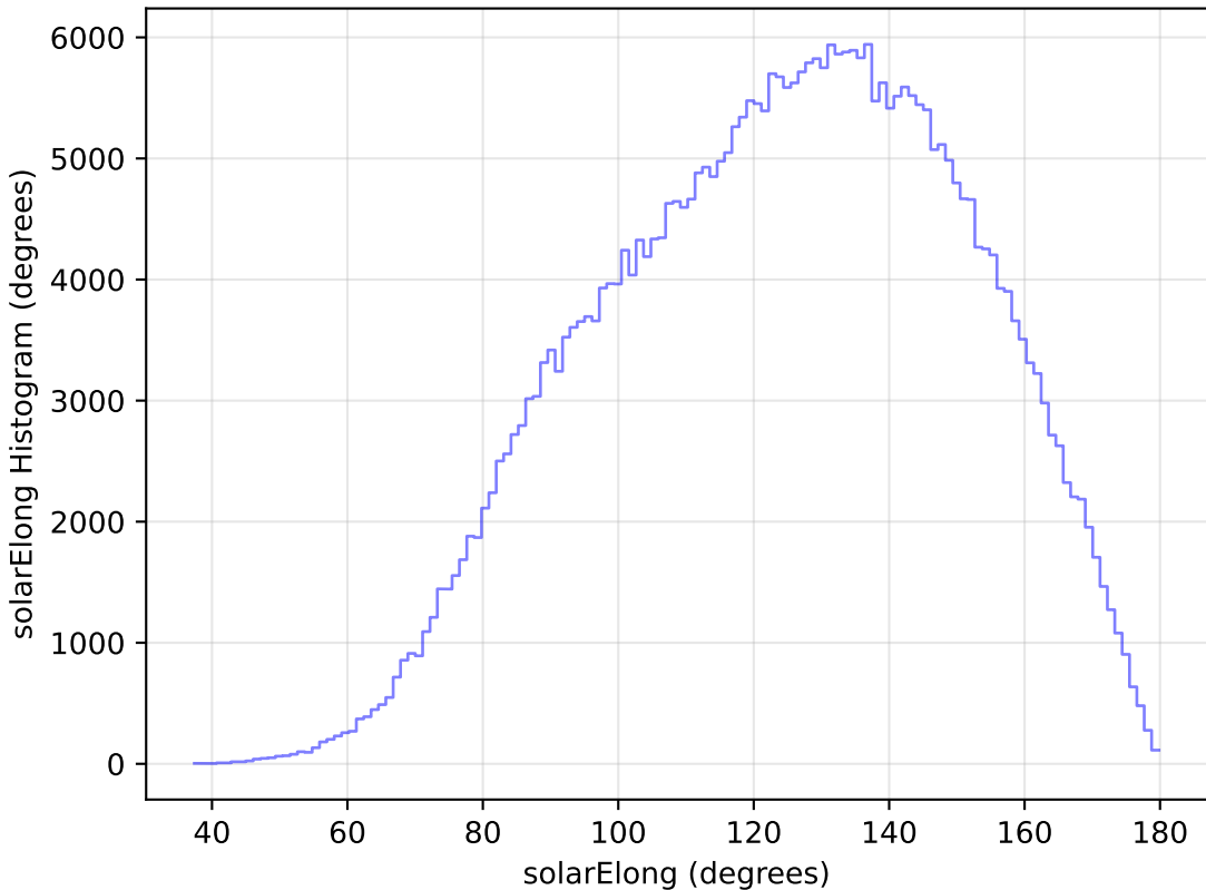
too_elab_r64_d2_giz_v3.4_10yrs All sky y band: solarElong Histogram
