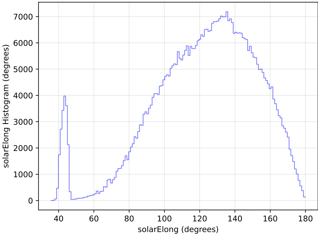
too_elab_r64_d2_giz_v3.4_10yrs All sky r band: solarElong Histogram
