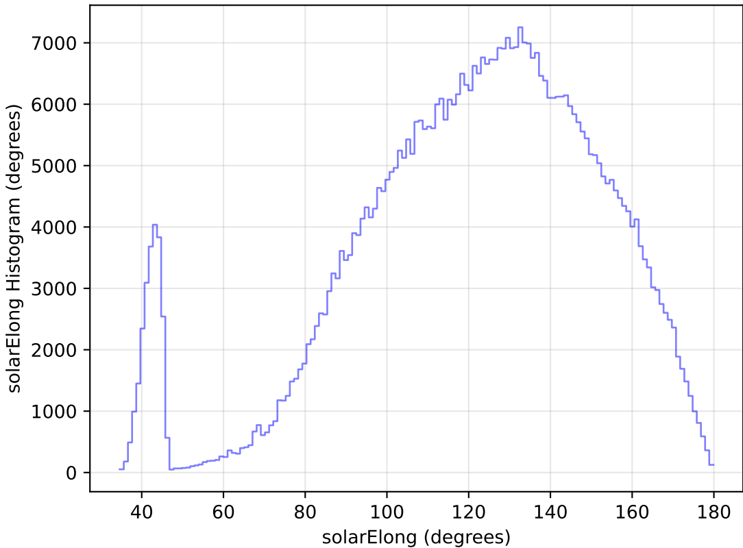
too_elab_r64_d2_giz_v3.4_10yrs All sky i band: solarElong Histogram
