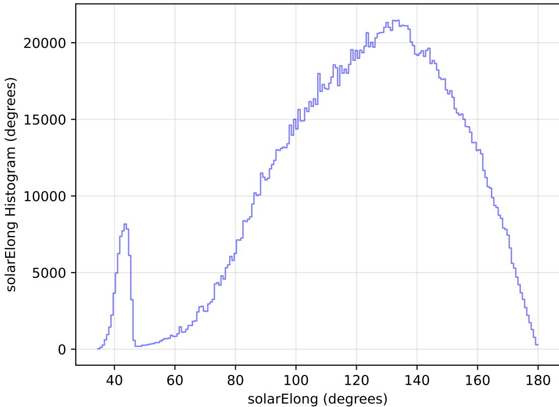
too_elab_r64_d2_giz_v3.4_10yrs All sky all bands: solarElong Histogram
