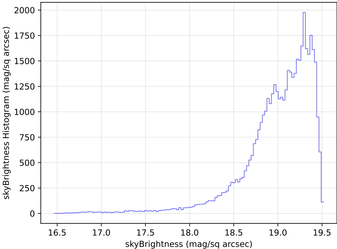
too_elab_r64_d2_giz_v3.4_10yrs Yr 1 z band: skyBrightness Histogram
