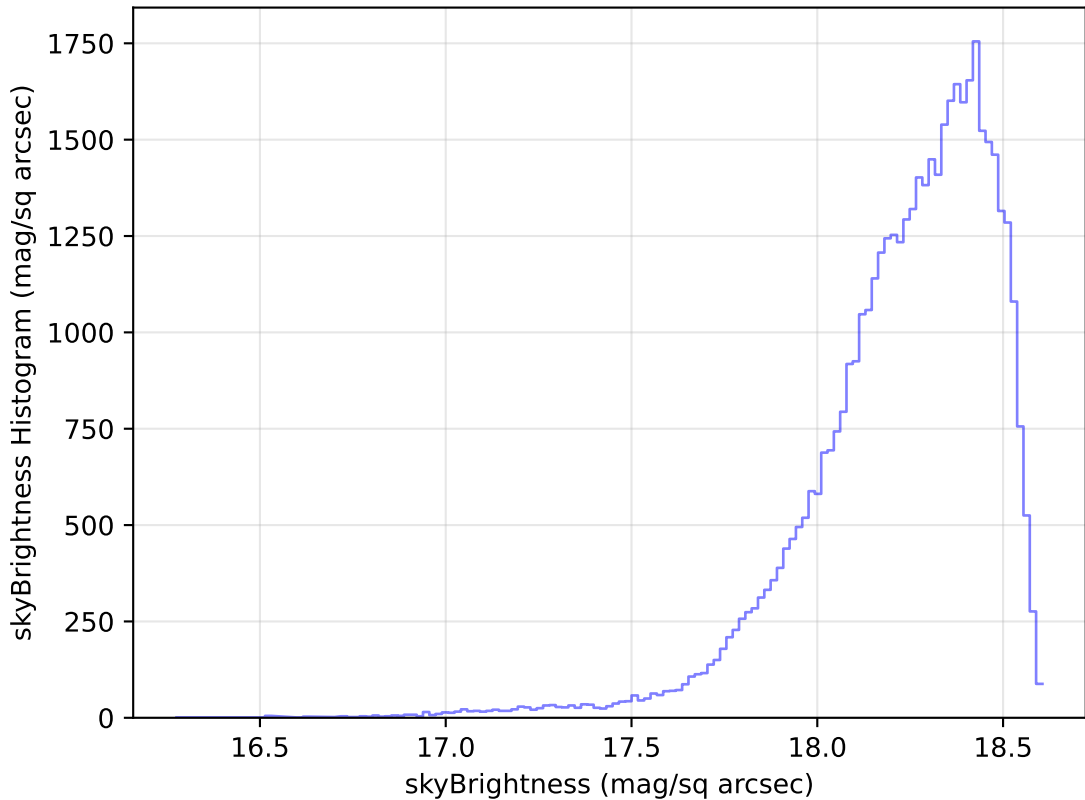
too_elab_r64_d2_giz_v3.4_10yrs Yr 1 y band: skyBrightness Histogram
