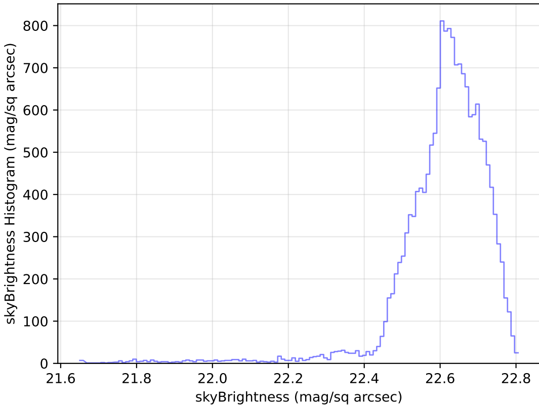
too_elab_r64_d2_giz_v3.4_10yrs Yr 1 u band: skyBrightness Histogram
