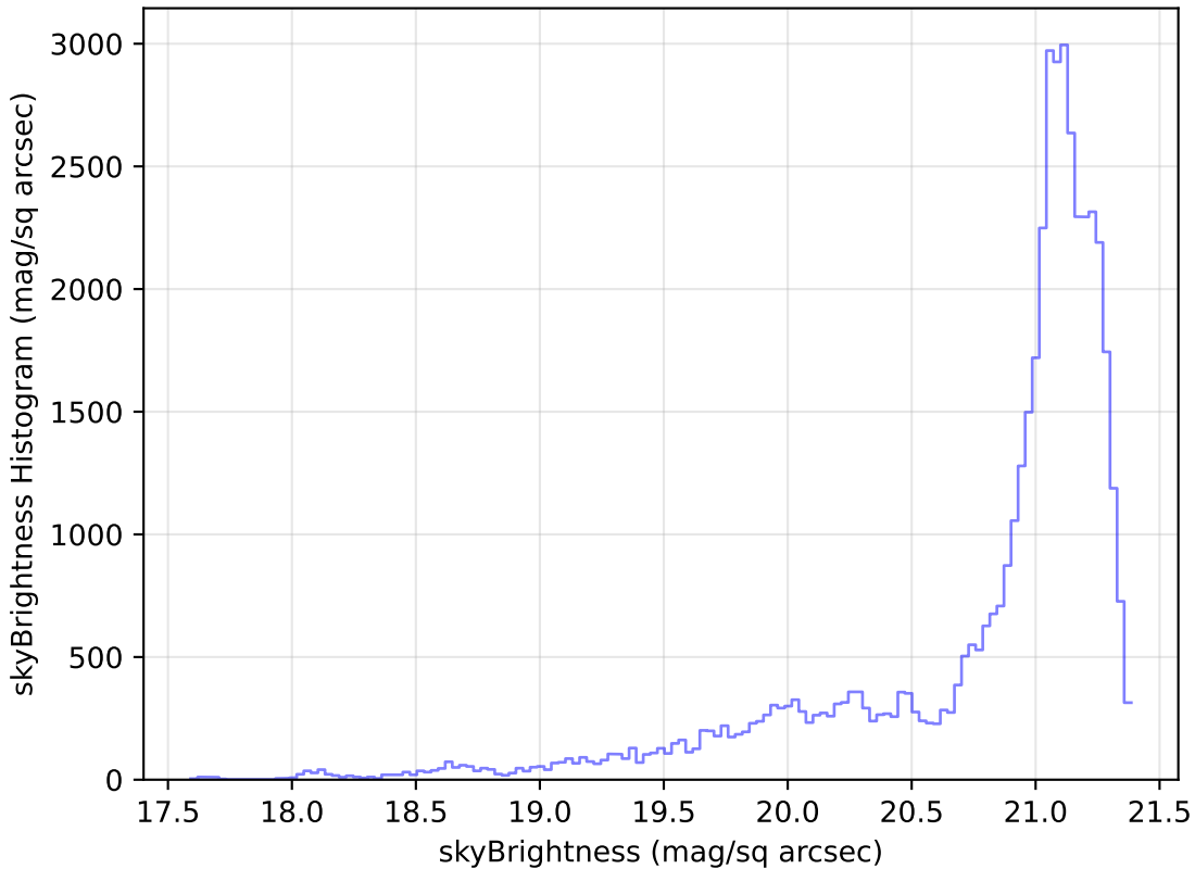
too_elab_r64_d2_giz_v3.4_10yrs Yr 1 r band: skyBrightness Histogram
