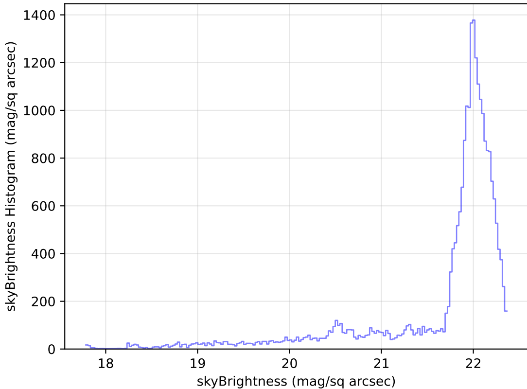
too_elab_r64_d2_giz_v3.4_10yrs Yr 1 g band: skyBrightness Histogram
