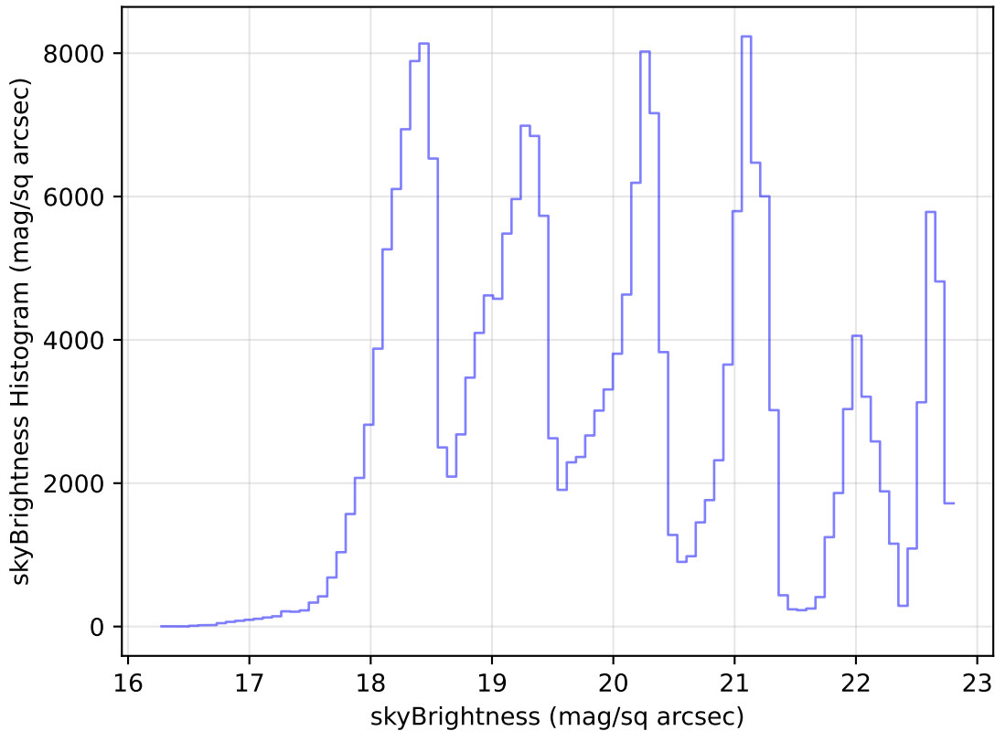
too_elab_r64_d2_giz_v3.4_10yrs Yr 1 all bands: skyBrightness Histogram
