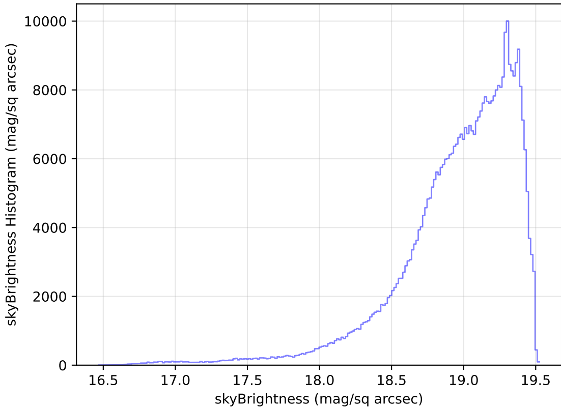
too_elab_r64_d2_giz_v3.4_10yrs WFD z band: skyBrightness Histogram
