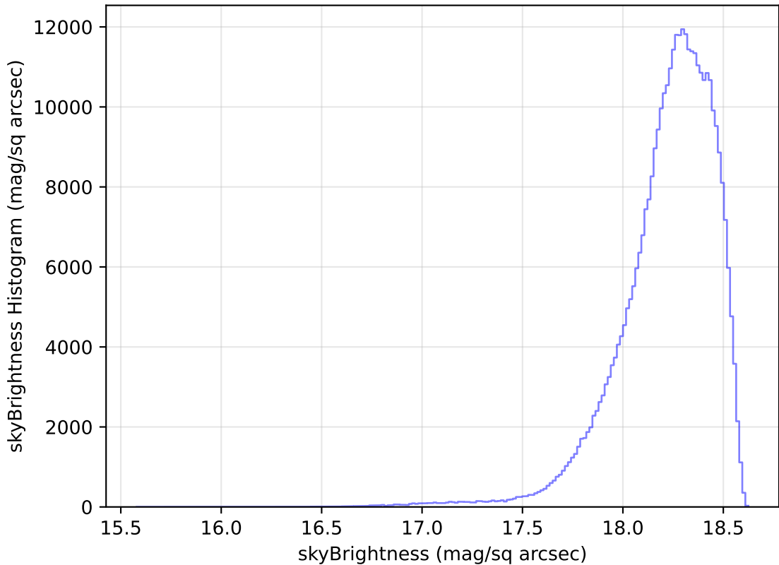
too_elab_r64_d2_giz_v3.4_10yrs WFD y band: skyBrightness Histogram
